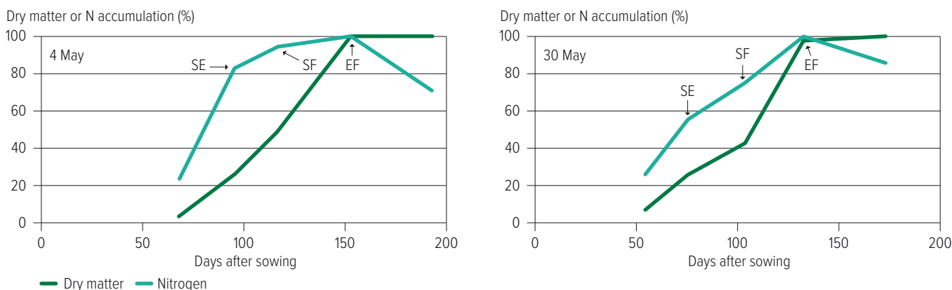
FIGURE 3-5 The relative accumulation of dry matter and N in canola at two sowing times and supplied with 75kg N/ha. The growth stages are stem elongation (SE), start of flowering (SF) and end of flowering (EF).
