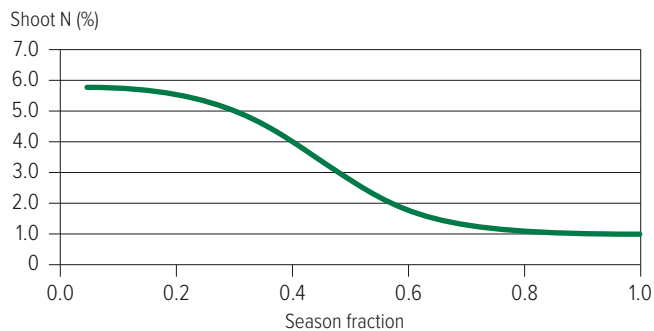
FIGURE 7-1 Approximate change in N concentration of wheat shoots during the life of an N sufficient crop. The value of 1 on the X-axis equates to crop maturity.
