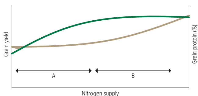
FIGURE 8-1 General response of yield (green line) and protein content (brown line) to N fertiliser.
