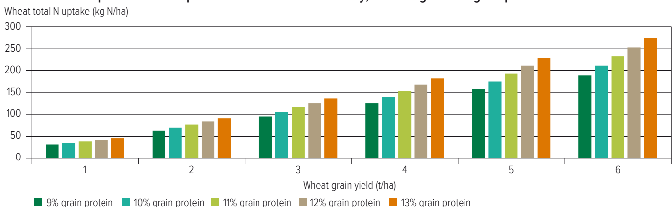
FIGURE 6-6 Wheat total N uptake (including roots) at a range of grain protein concentrations and grain yields. It is assumed that 70 per cent of total plant N is in the shoot at maturity, and that grain N is grain protein/5.7.
