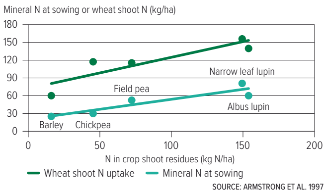
FIGURE 4-2 Relationships between the N in crop shoot residues and the soil mineral N at sowing of a following wheat crop and the uptake of N by the following wheat, Wagga Wagga, NSW.
