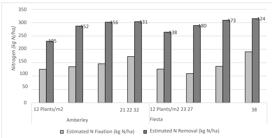
Figure 3. Estimates of nitrogen fixation and removal from high yielding irrigated faba bean crops. Data labels show the nitrogen deficit.
