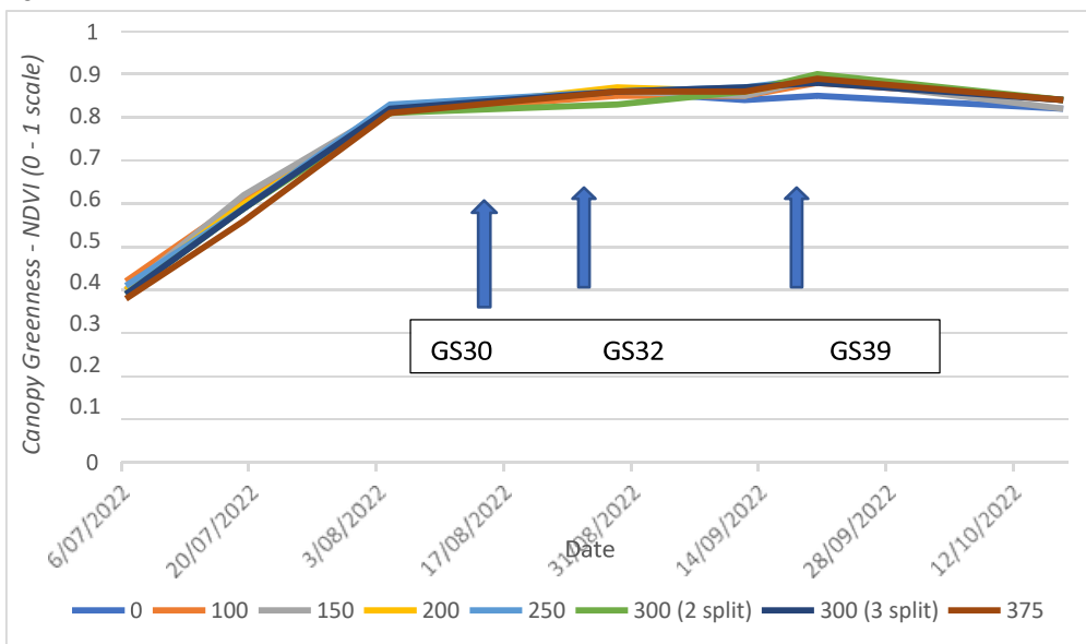
Figure 4. Influence of applied N rates and timing on crop reflectance measured using NDVI – Frances, SA 2021 & 2022 cv Rockstar.
